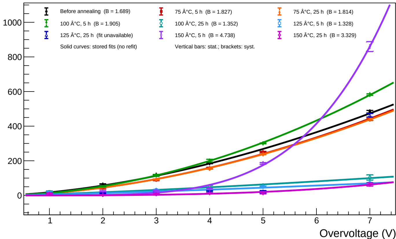
A1_T=20 - Spot 27 (x = 1048.43, y = 957.20): luminosity vs overvoltage for all annealing phases
