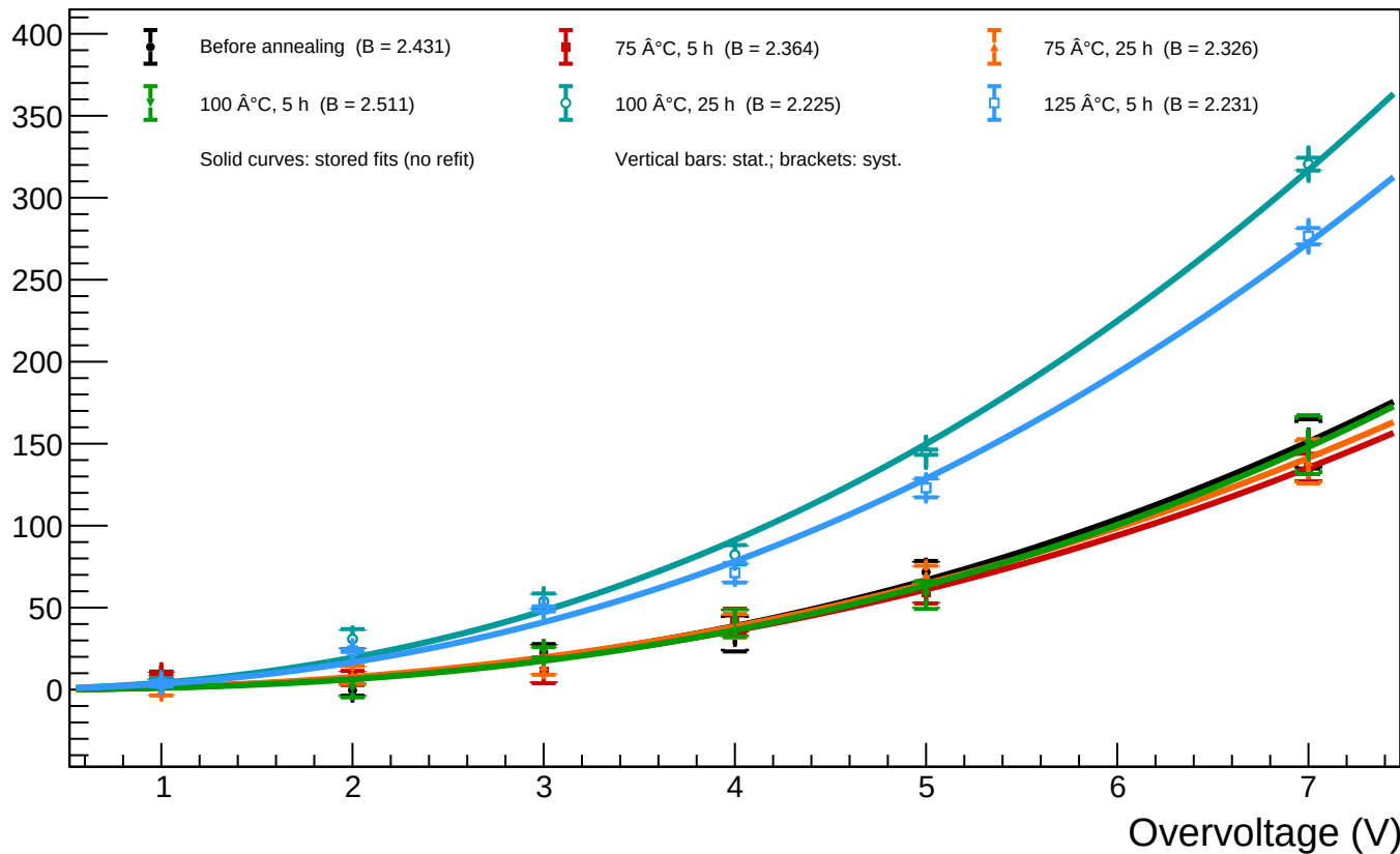
A1_T=20 - Spot 28 (x = 1051.57, y = 804.29): luminosity vs overvoltage for all annealing phases
