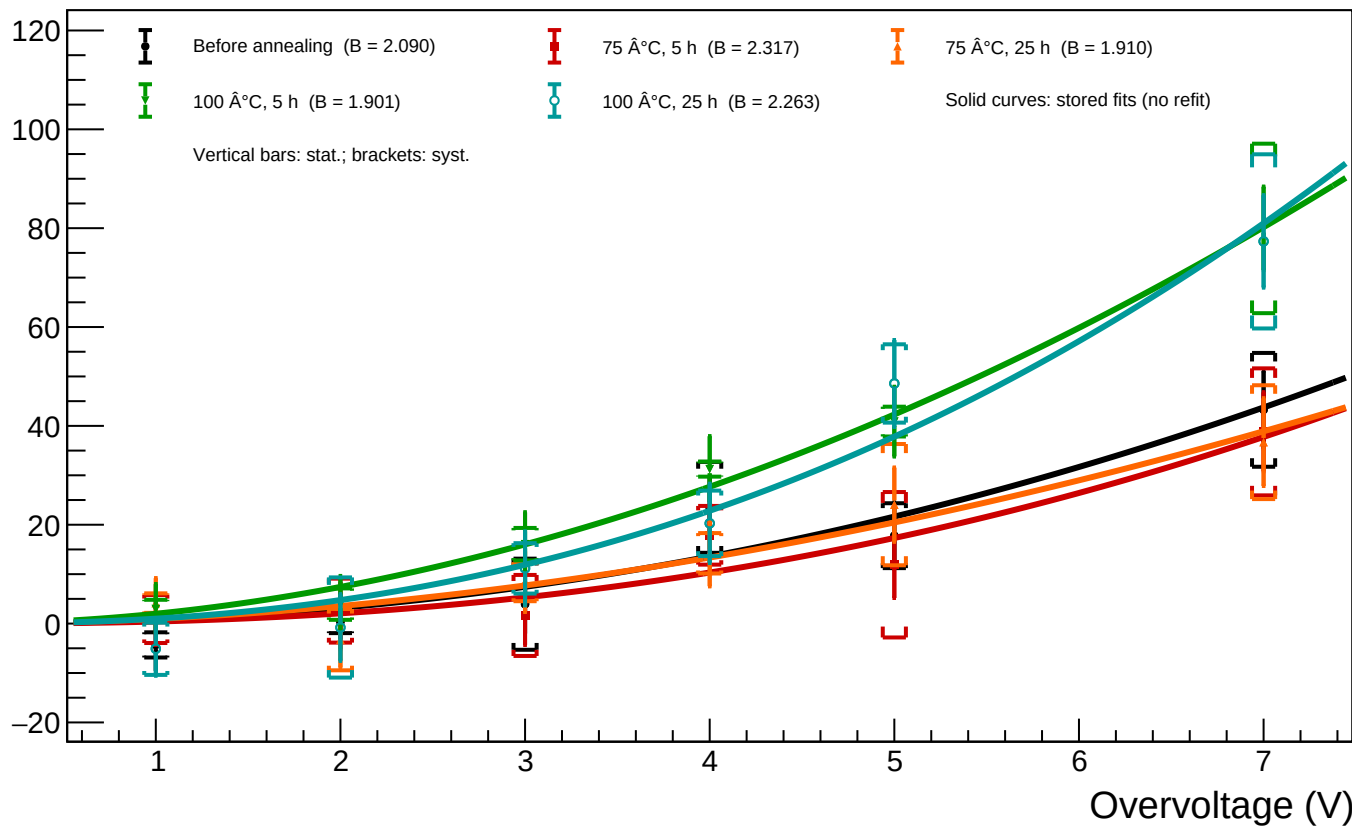
A1_T=20 - Spot 29 (x = 1068.29, y = 234.46): luminosity vs overvoltage for all annealing phases
