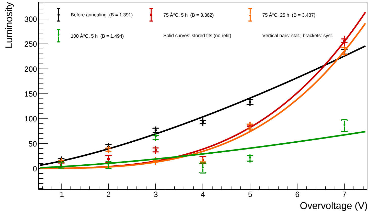
A1_T=20 - Spot 30 (x = 1088.01, y = 910.26): luminosity vs overvoltage for all annealing phases
