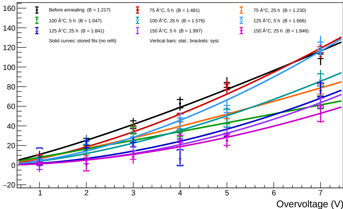
A1_T=20 - Spot 32 (x = 1148.87, y = 429.04): luminosity vs overvoltage for all annealing phases
