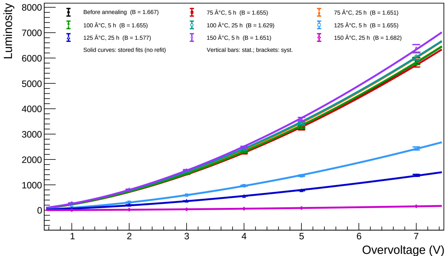
A1_T=20 - Spot 33 (x = 1169.52, y = 239.79): luminosity vs overvoltage for all annealing phases
