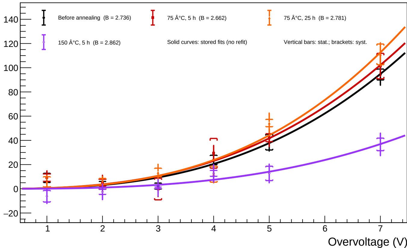
A1_T=20 - Spot 34 (x = 1180.58, y = 593.45): luminosity vs overvoltage for all annealing phases
