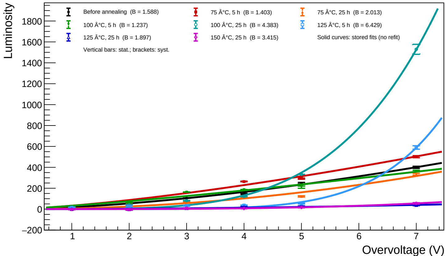
A1_T=20 - Spot 37 (x = 1244.59, y = 484.33): luminosity vs overvoltage for all annealing phases
