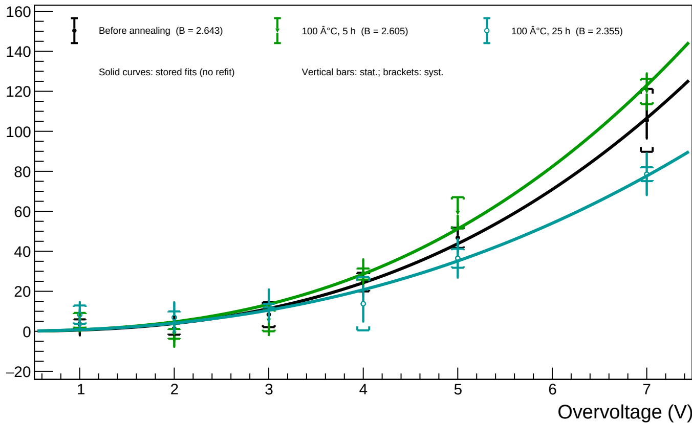
A1_T=20 - Spot 38 (x = 1254.72, y = 595.84): luminosity vs overvoltage for all annealing phases
