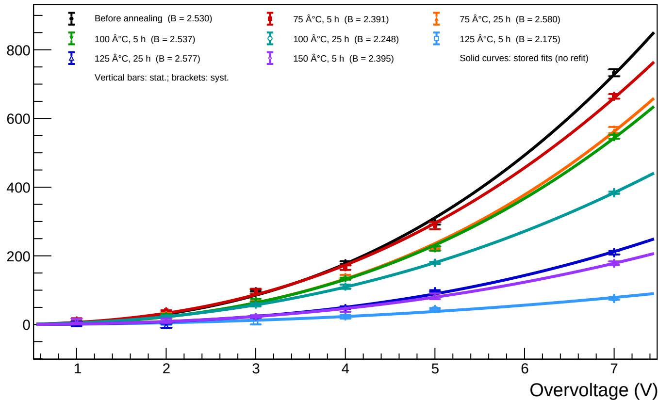
A1_T=20 - Spot 4 (x = 193.71, y = 520.08): luminosity vs overvoltage for all annealing phases
