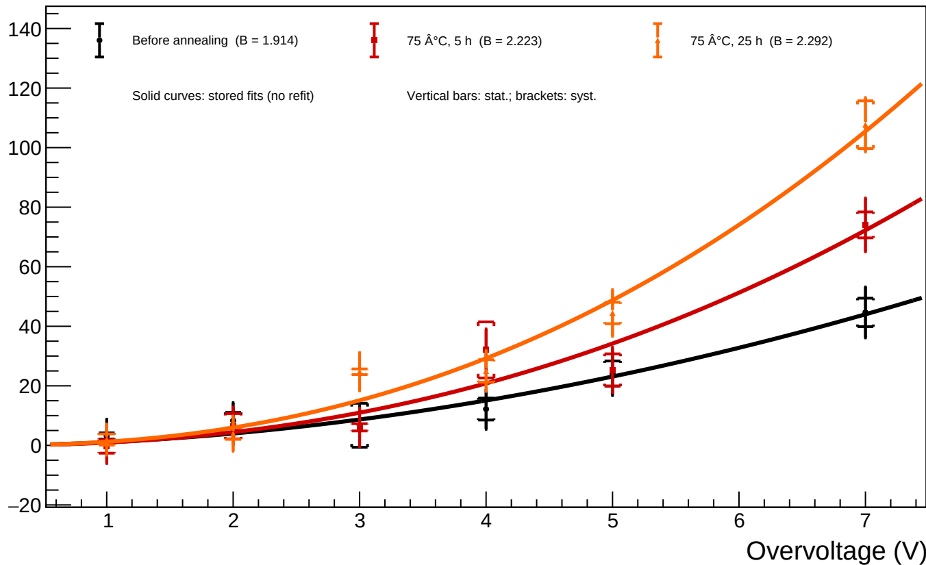
A1_T=20 - Spot 44 (x = 1322.15, y = 529.60): luminosity vs overvoltage for all annealing phases
