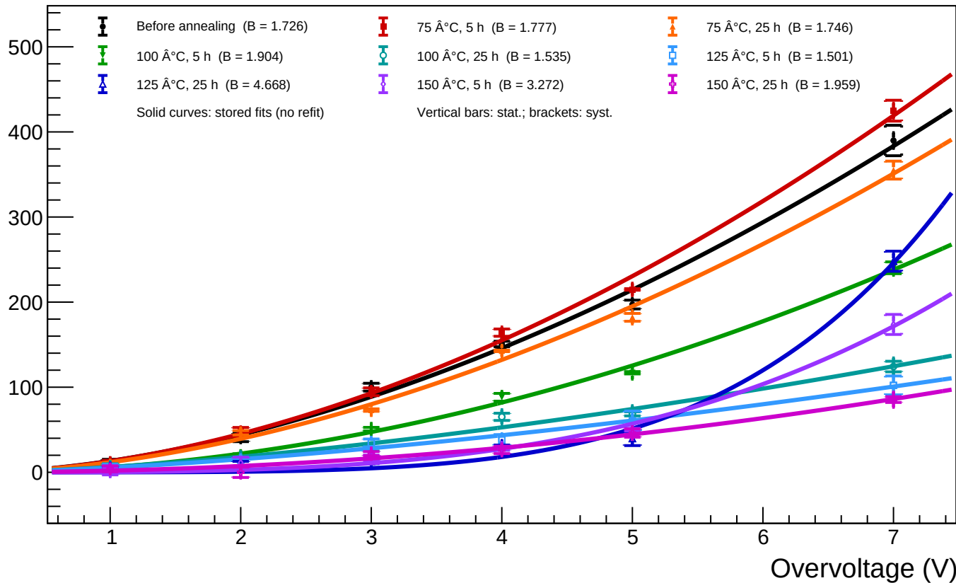
A1_T=20 - Spot 45 (x = 1372.43, y = 811.18): luminosity vs overvoltage for all annealing phases
