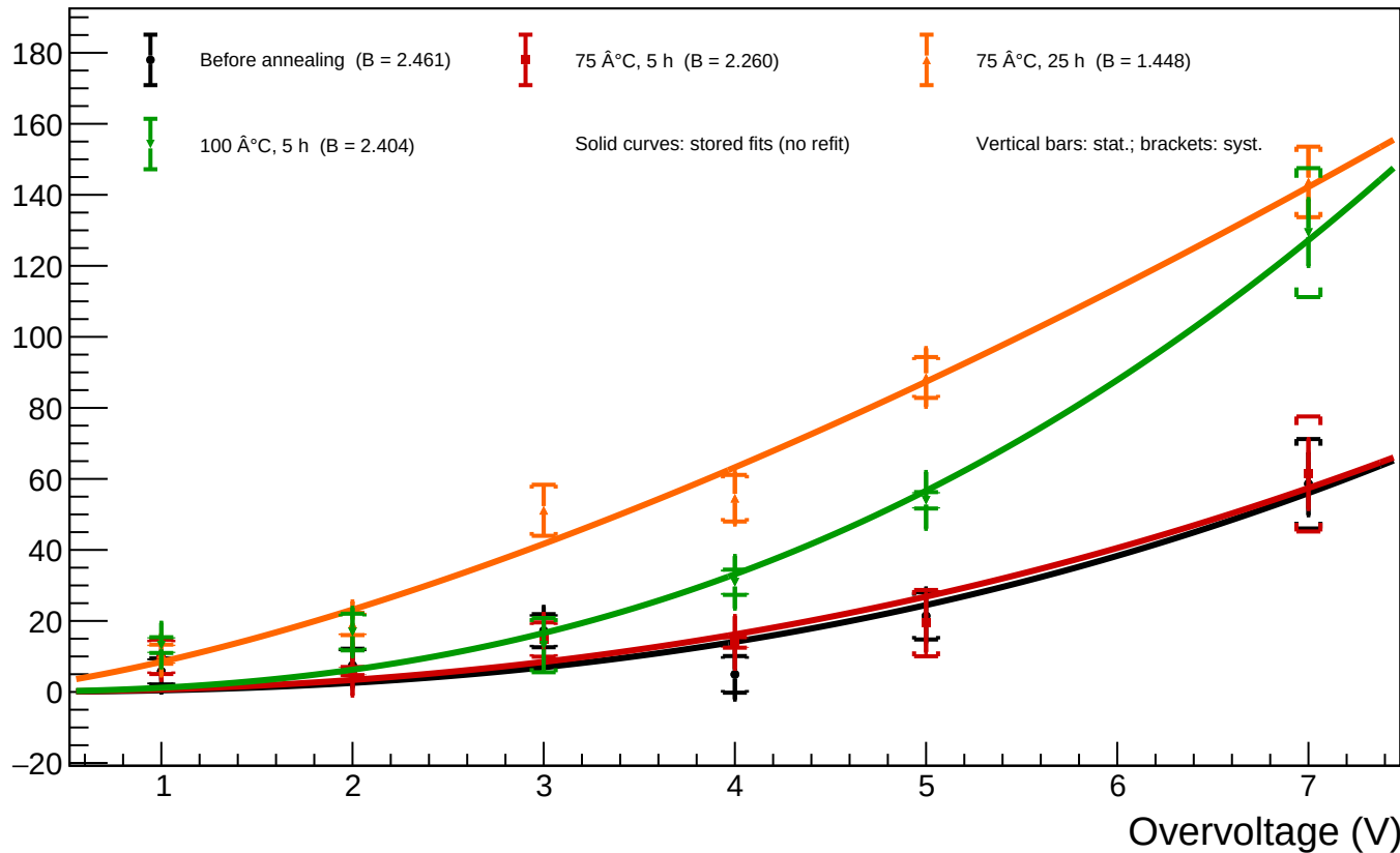
A1_T=20 - Spot 47 (x = 1465.47, y = 945.43): luminosity vs overvoltage for all annealing phases
