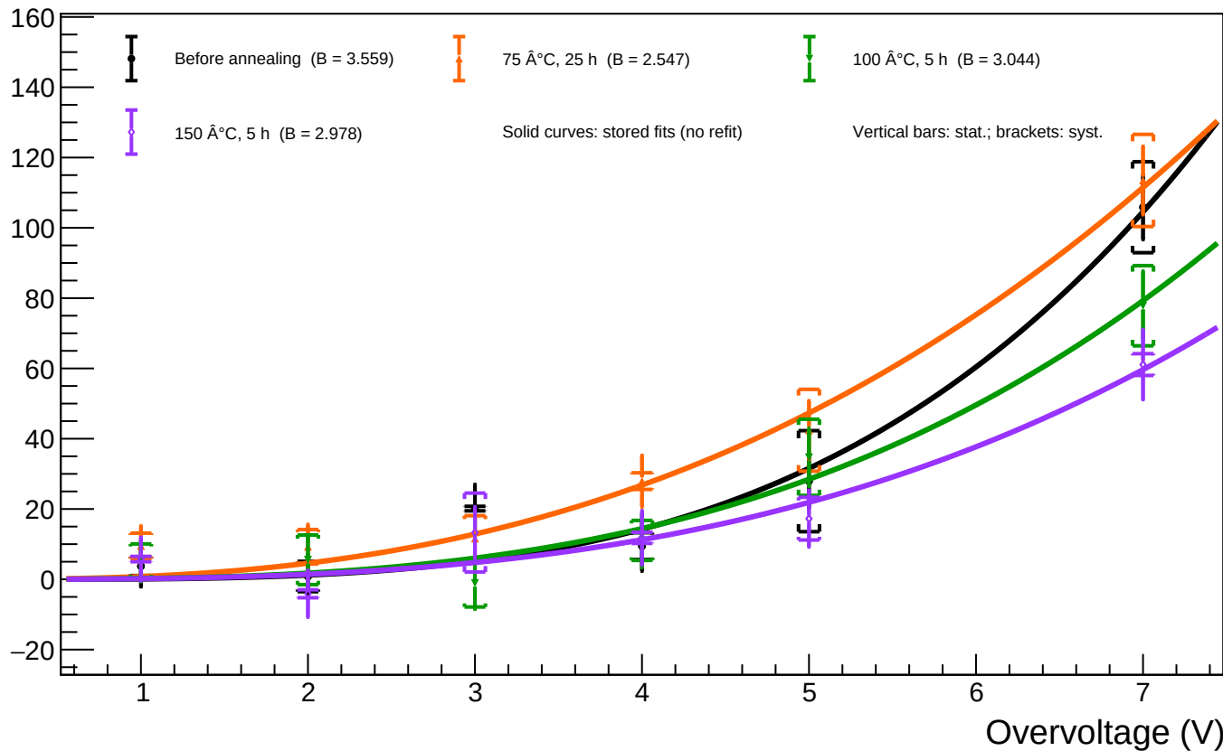
A1_T=20 - Spot 5 (x = 232.08, y = 757.48): luminosity vs overvoltage for all annealing phases
