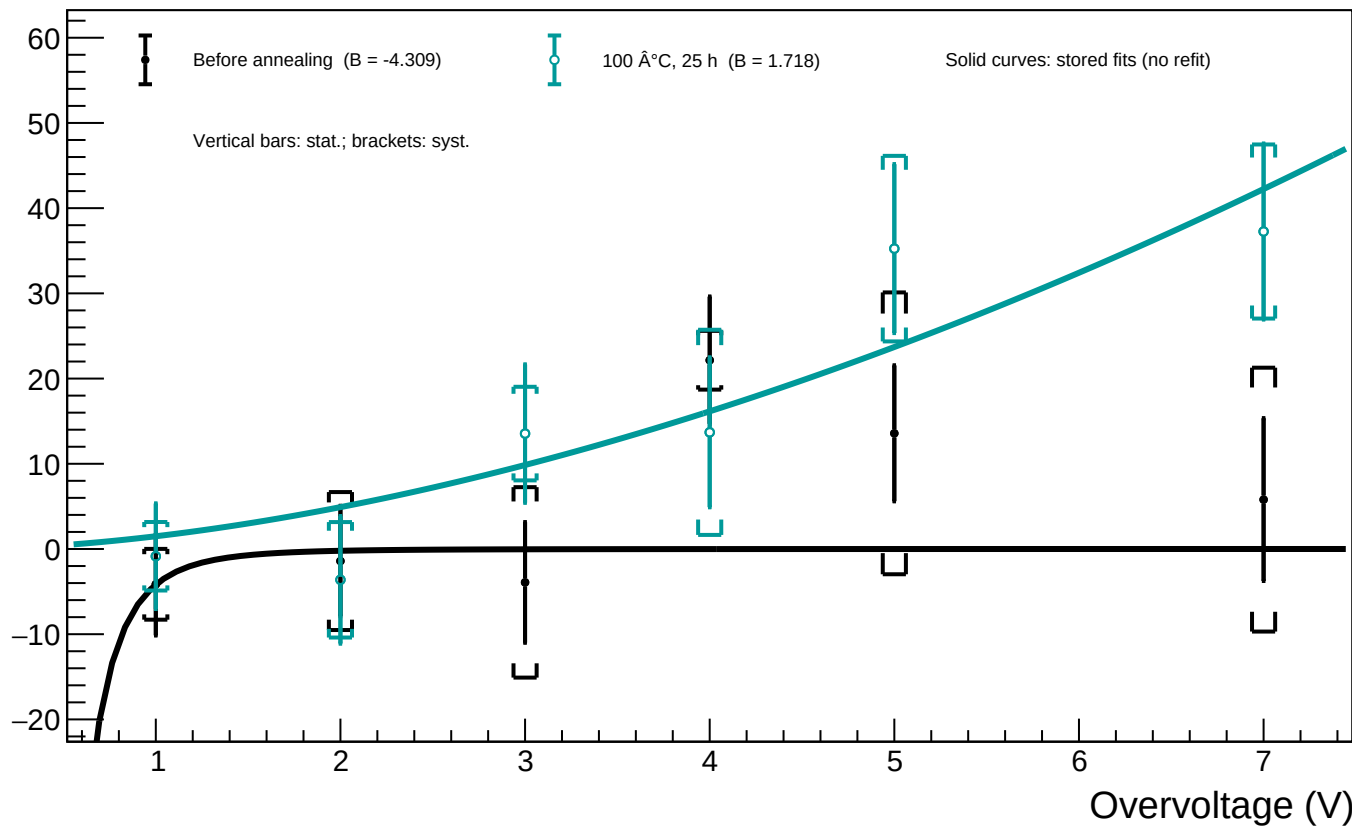
A1_T=20 - Spot 52 (x = 1596.82, y = 321.11): luminosity vs overvoltage for all annealing phases
