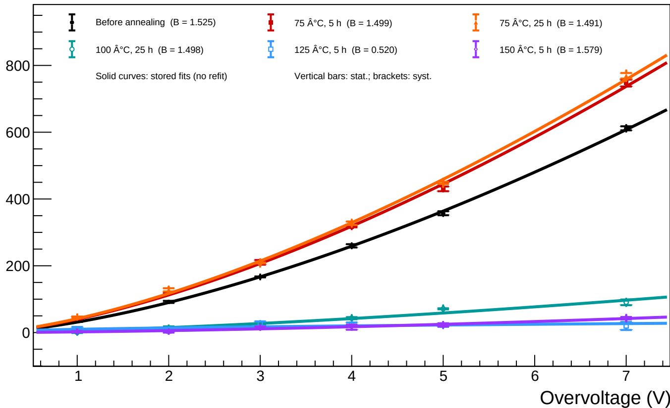
A1_T=20 - Spot 55 (x = 1772.47, y = 478.77): luminosity vs overvoltage for all annealing phases
