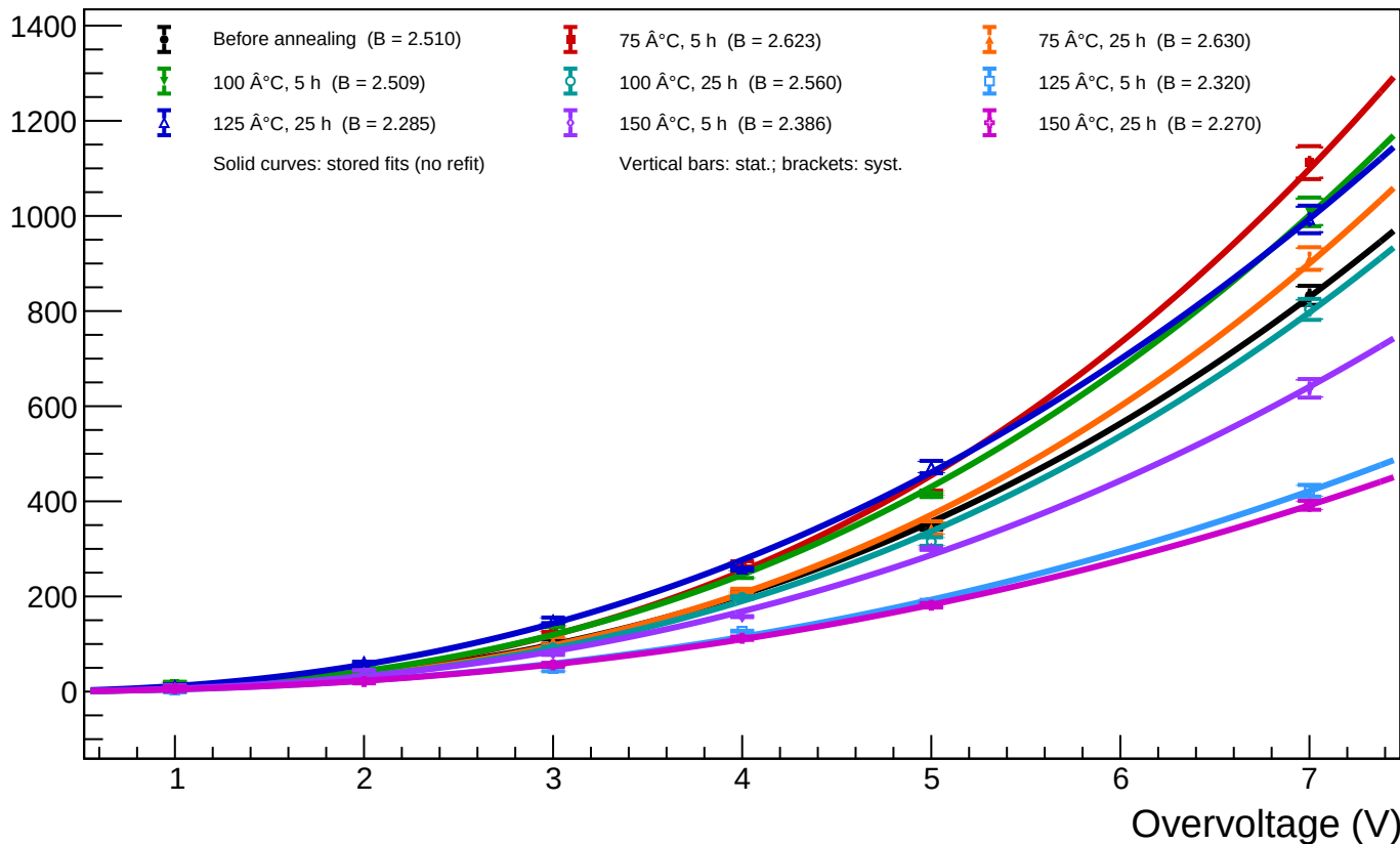
A1_T=20 - Spot 57 (x = 1820.88, y = 357.33): luminosity vs overvoltage for all annealing phases
