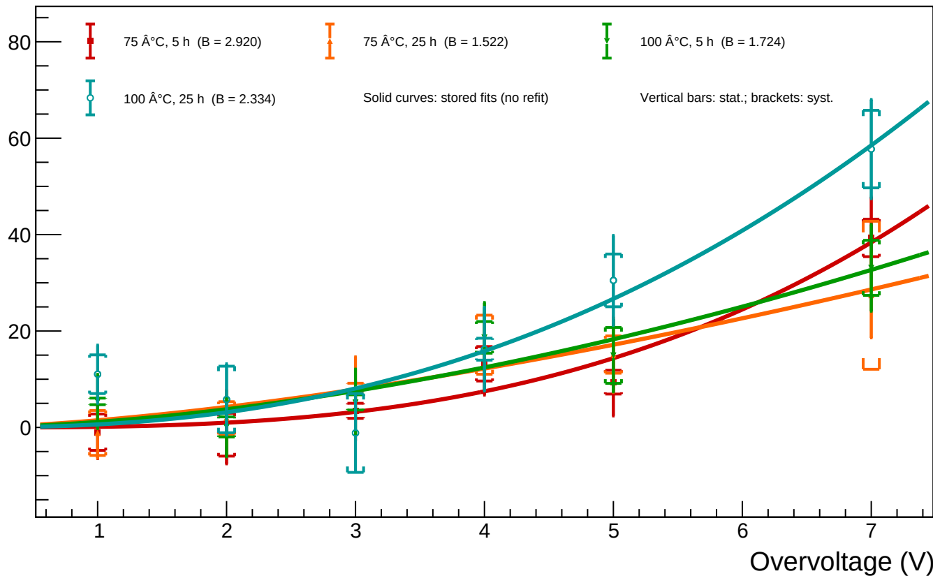
A1_T=20 - Spot 60 (x = 1655.07, y = 493.38): luminosity vs overvoltage for all annealing phases
