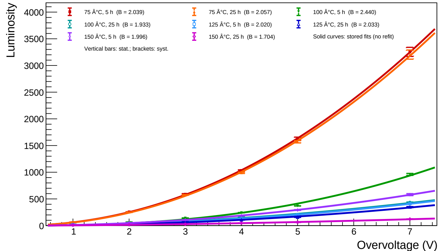
A1_T=20 - Spot 62 (x = 513.87, y = 881.63): luminosity vs overvoltage for all annealing phases
