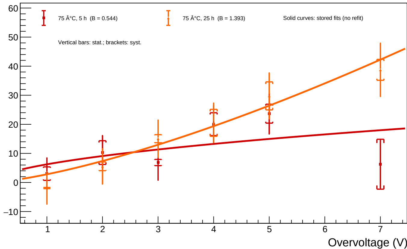
A1_T=20 - Spot 63 ( x = 899.09 , y = 256.42 ): luminosity vs overvoltage for all annealing phases
