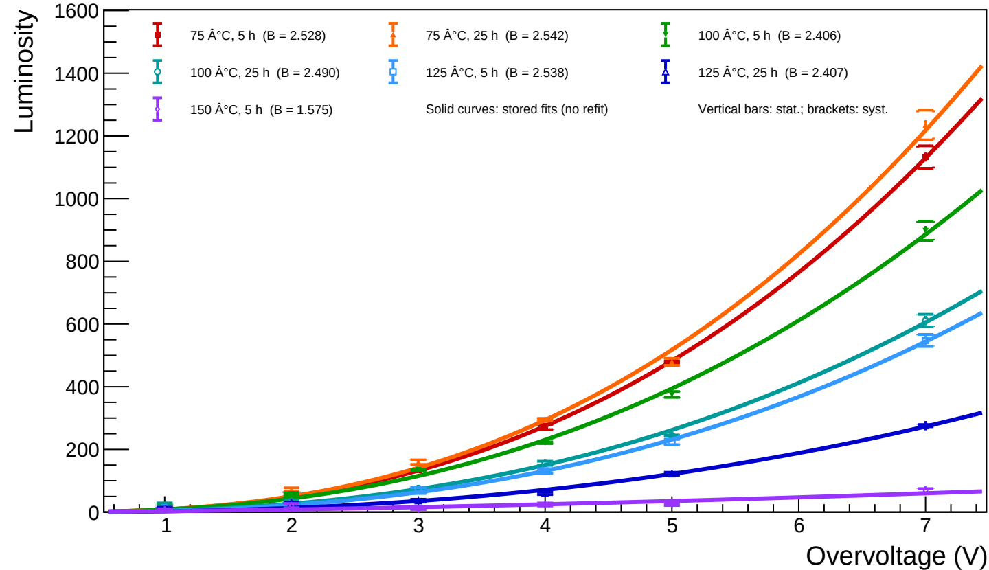
A1_T=20 - Spot 64 ( x = 907.53 , y = 731.13 ): luminosity vs overvoltage for all annealing phases
