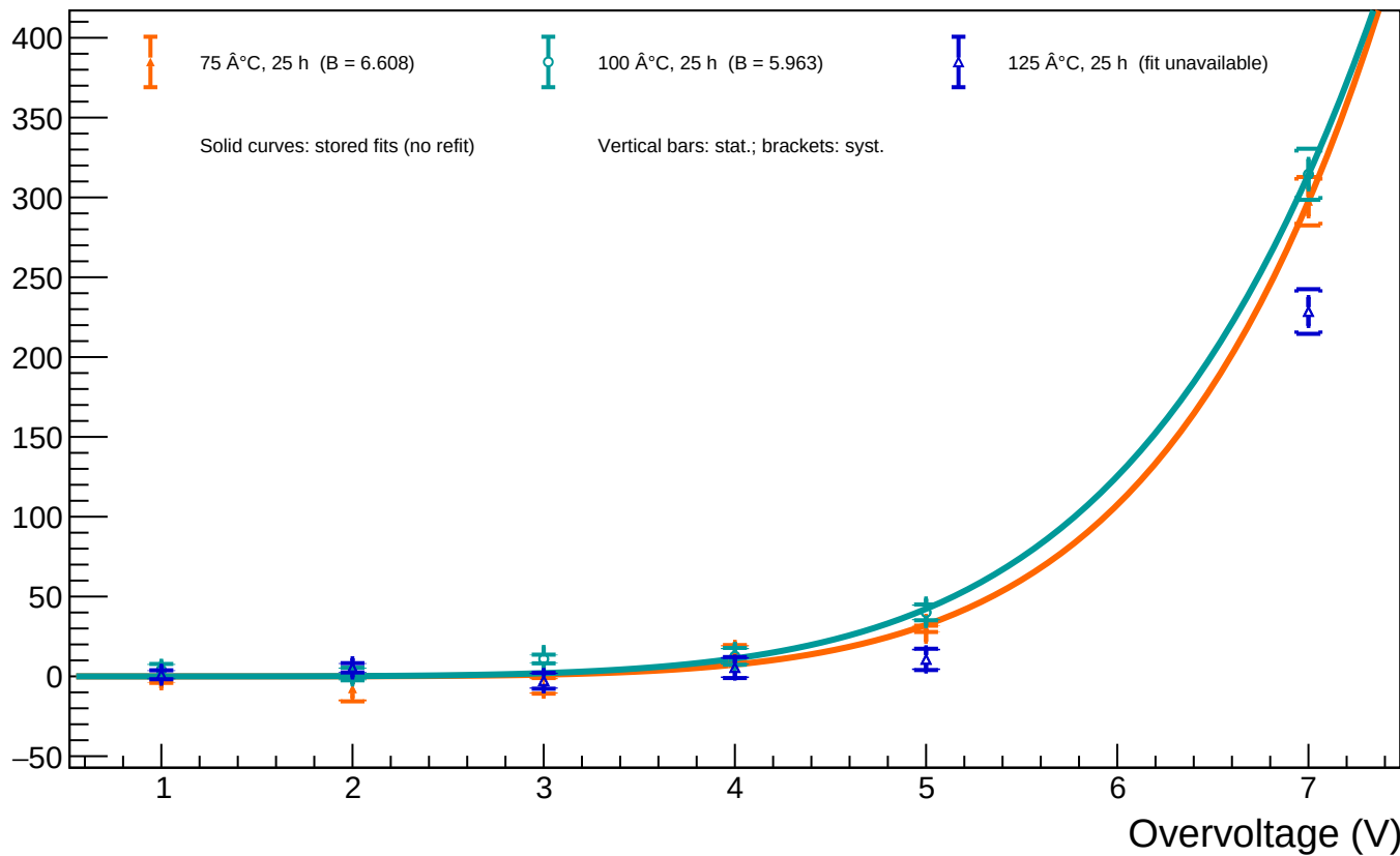
A1_T=20 - Spot 66 ( x = 586.20 , y = 494.22 ): luminosity vs overvoltage for all annealing phases
