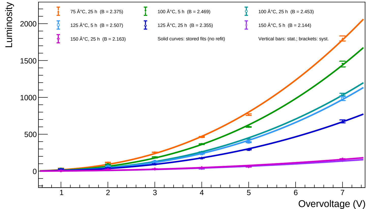
A1_T=20 - Spot 67 (x = 1616.34, y = 987.45): luminosity vs overvoltage for all annealing phases
