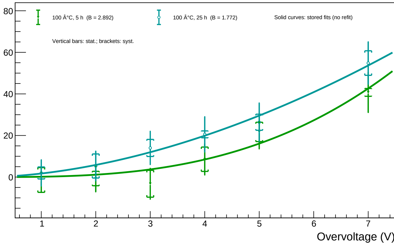
A1_T=20 - Spot 68 ( x = 262.91 , y = 495.09 ): luminosity vs overvoltage for all annealing phases
