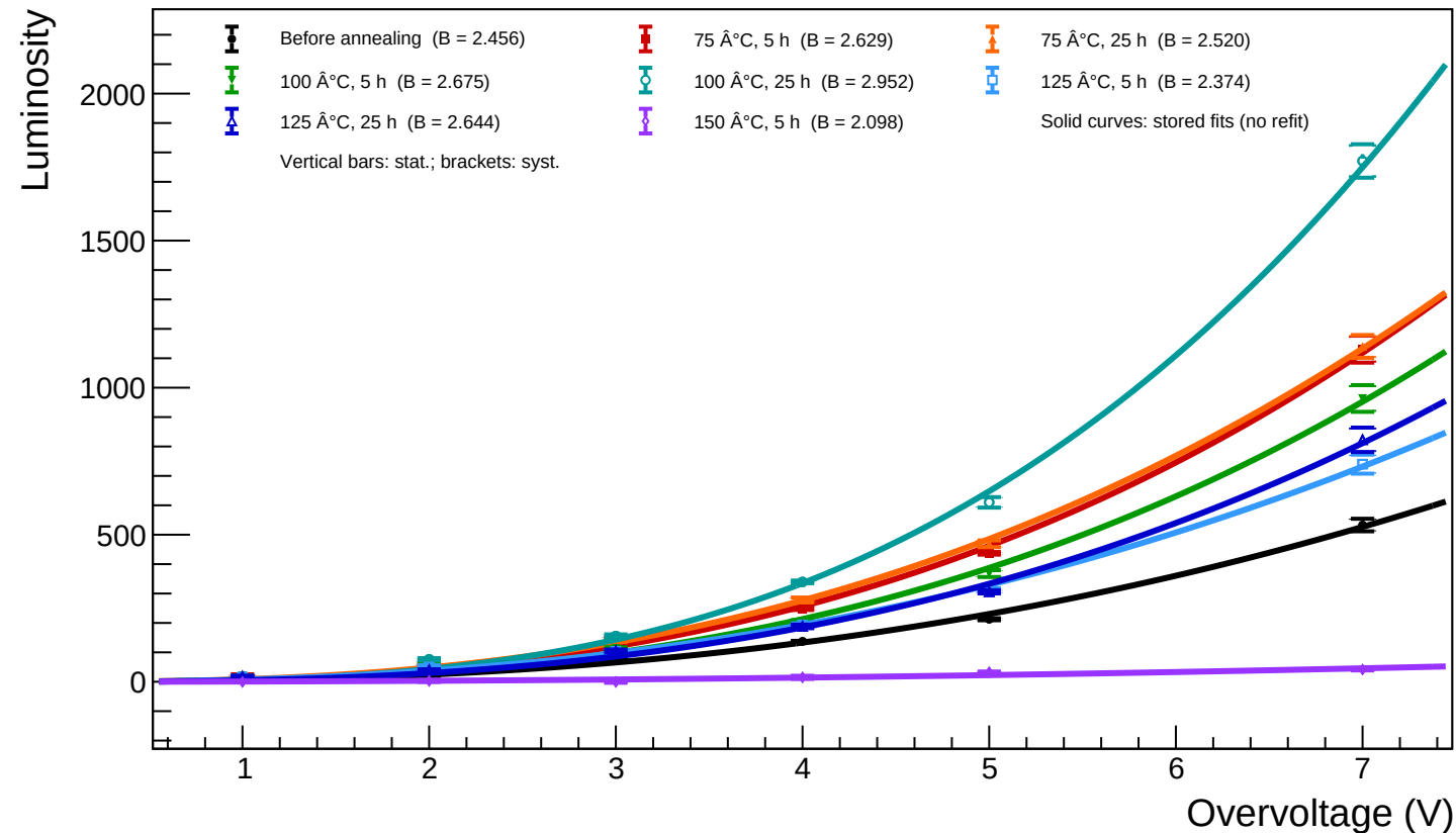
A1_T=20 - Spot 7 (x = 253.67, y = 351.34): luminosity vs overvoltage for all annealing phases
