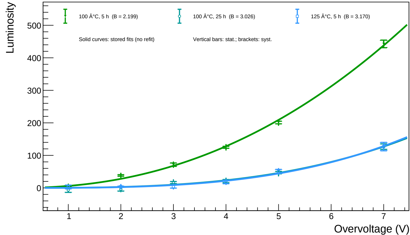
A1_T=20 - Spot 72 (x = 1403.83, y = 206.32): luminosity vs overvoltage for all annealing phases
