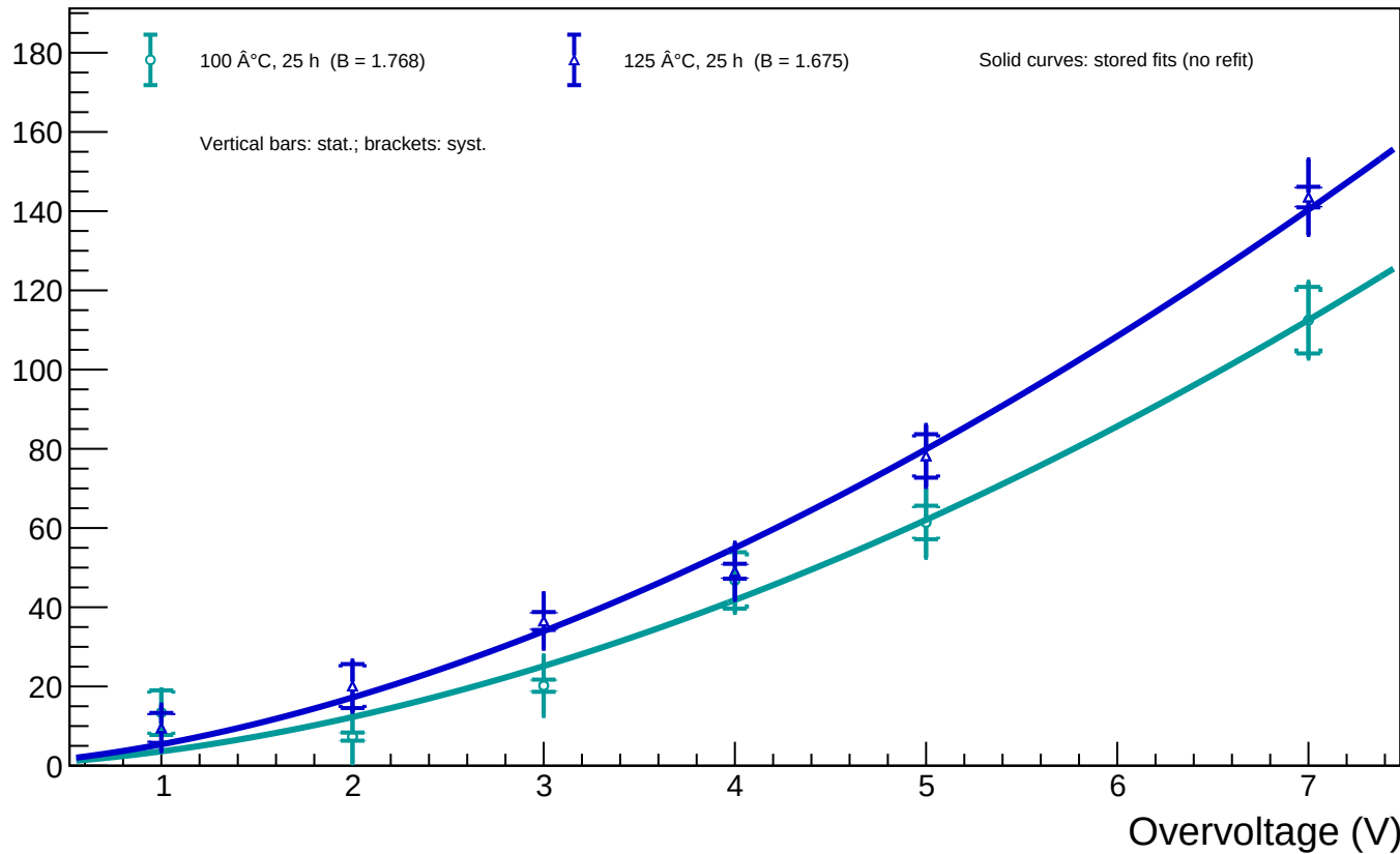
A1_T=20 - Spot 75 ( x = 859.37 , y = 472.75 ): luminosity vs overvoltage for all annealing phases
