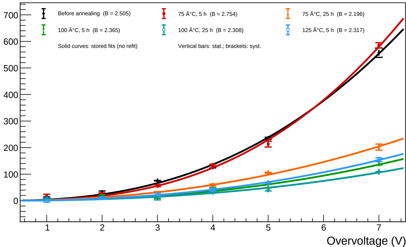
A1_T=20 - Spot 8 (x = 356.70, y = 846.98): luminosity vs overvoltage for all annealing phases
