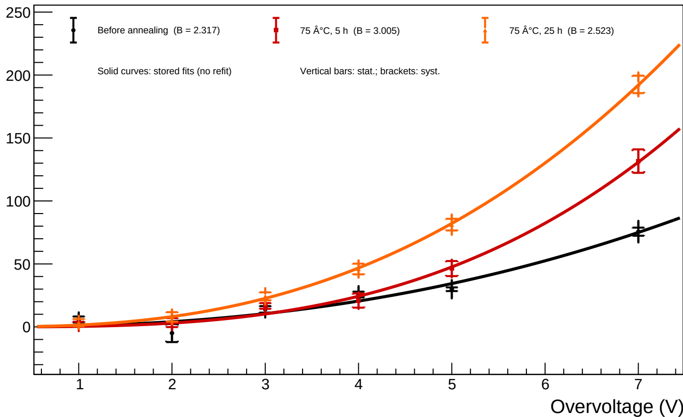
A1_T=20 - Spot 9 (x = 375.23, y = 369.88): luminosity vs overvoltage for all annealing phases
