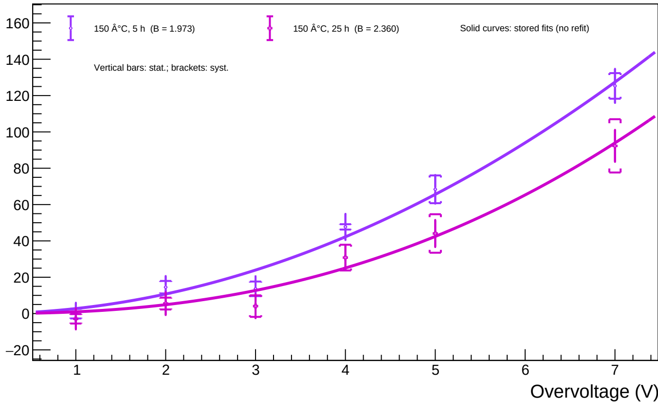
A1_T=20 - Spot 92 (x = 1769.29, y = 209.41): luminosity vs overvoltage for all annealing phases
