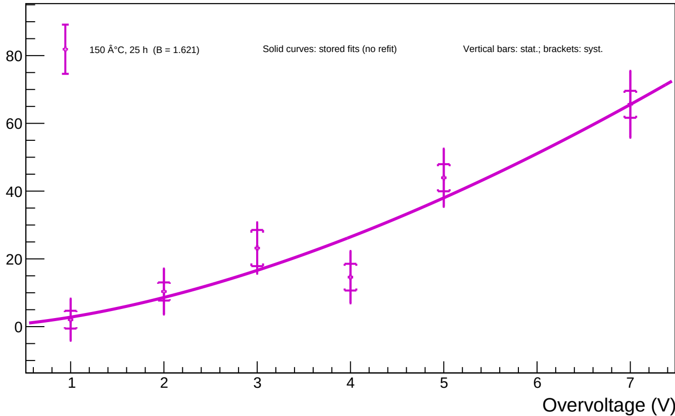
A1_T=20 - Spot 95 ( x = 806.23 , y = 190.86 ): luminosity vs overvoltage for all annealing phases
