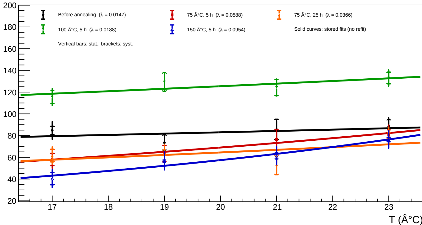
A1_v=5 - Spot 1 (x = 80.91, y = 94.55): luminosity vs temperature for all annealing phases
