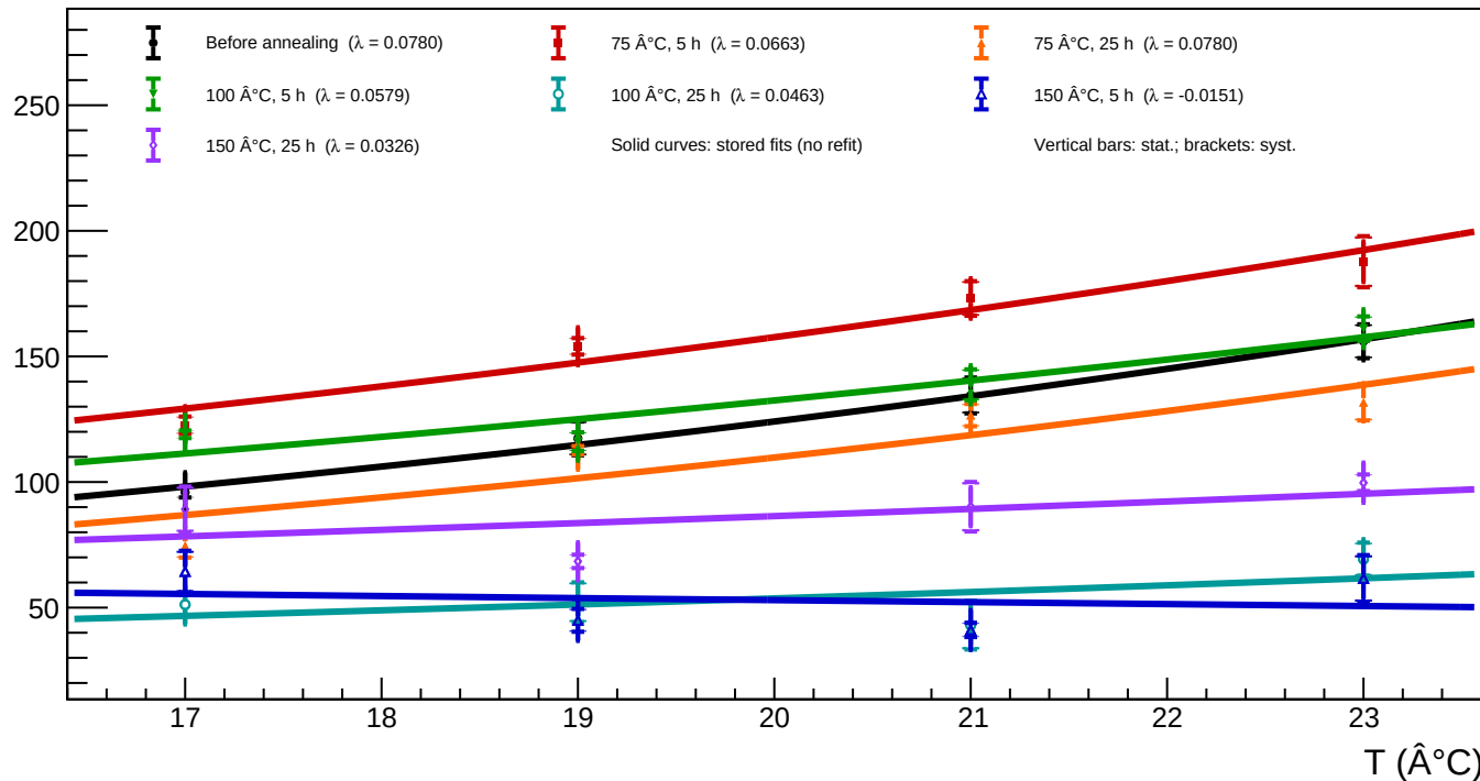
A1_v=5 - Spot 12 (x = 425.98, y = 71.48): luminosity vs temperature for all annealing phases
