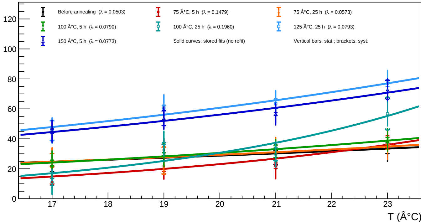
A1_v=5 - Spot 14 ( x = 573.41 , y = 121.23 ): luminosity vs temperature for all annealing phases
