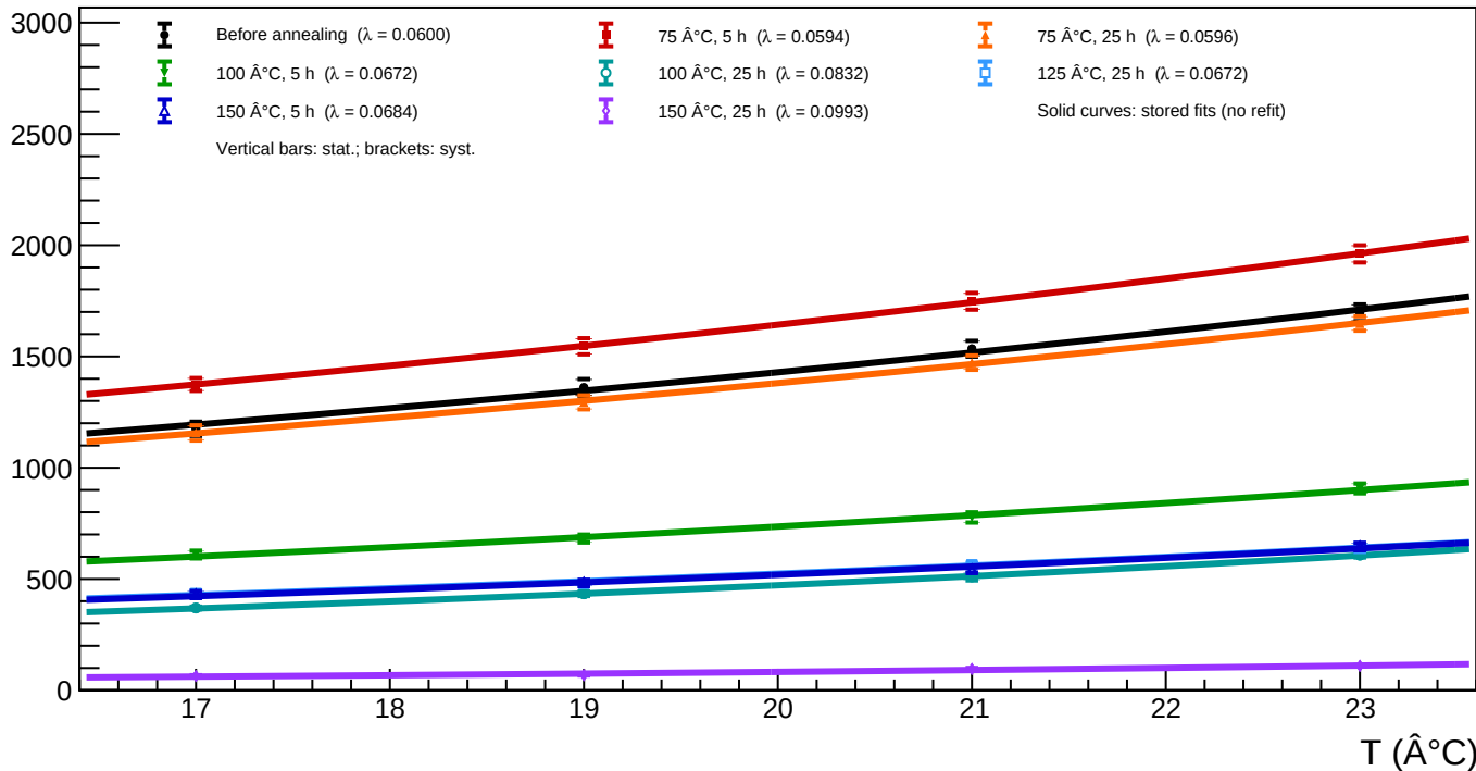
A1_v=5 - Spot 18 (x = 649.83, y = 572.61): luminosity vs temperature for all annealing phases
