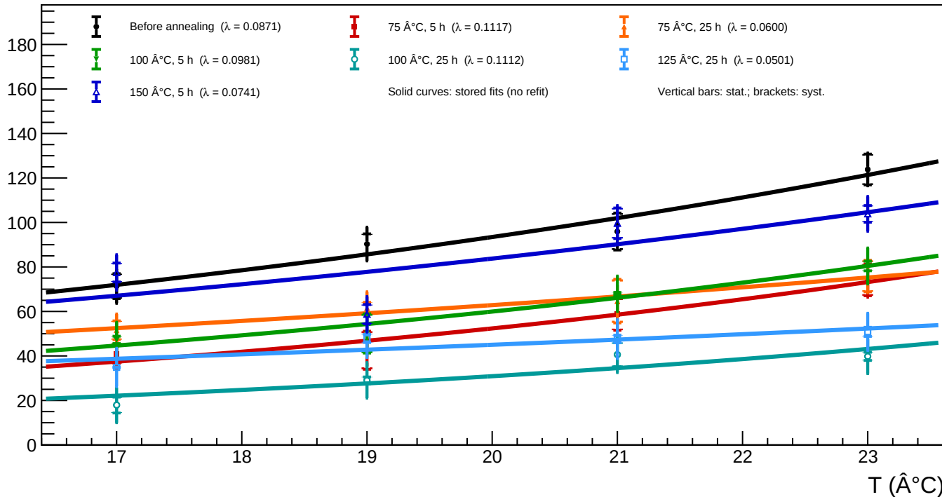
A1_v=5 - Spot 19 (x = 660.93, y = 686.94): luminosity vs temperature for all annealing phases
