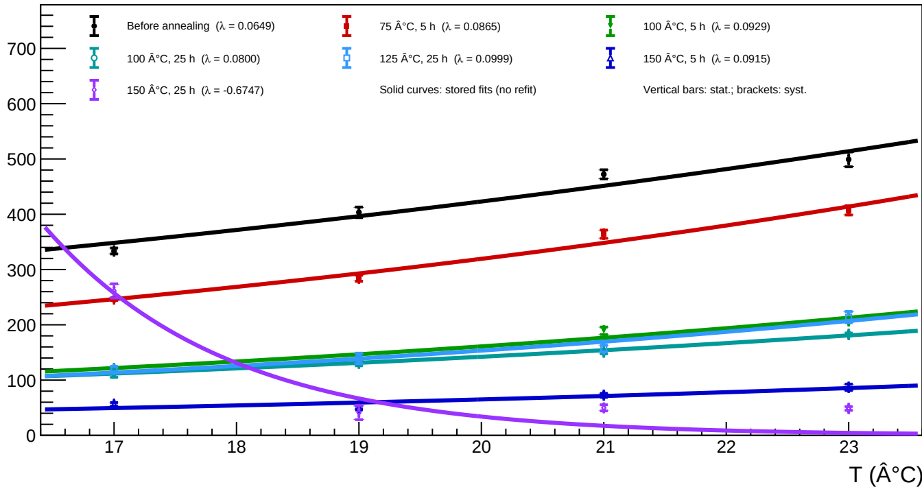
A1_v=5 - Spot 22 (x = 808.06, y = 586.31): luminosity vs temperature for all annealing phases
