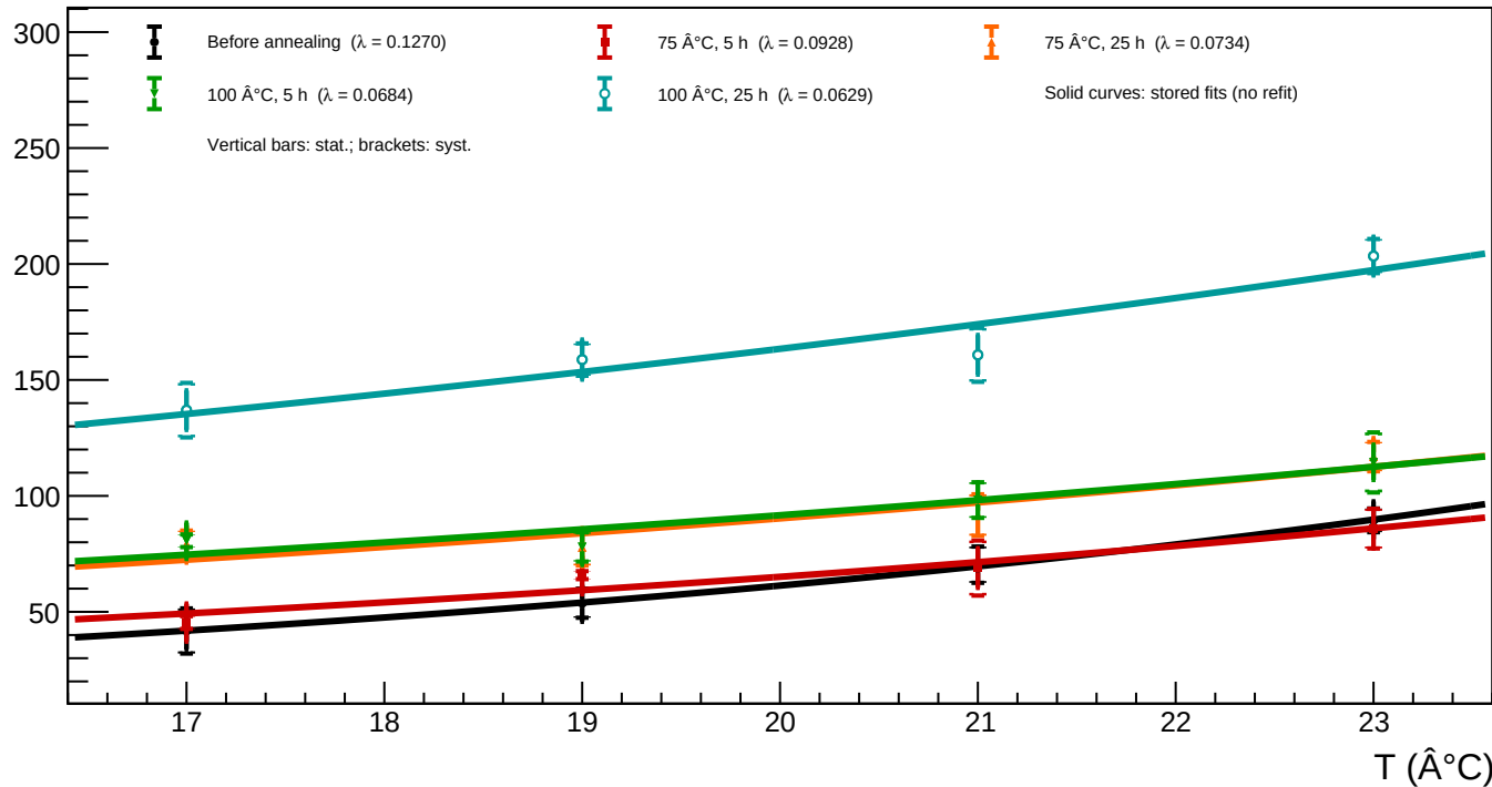
A1_v=5 - Spot 23 (x = 816.50, y = 314.06): luminosity vs temperature for all annealing phases
