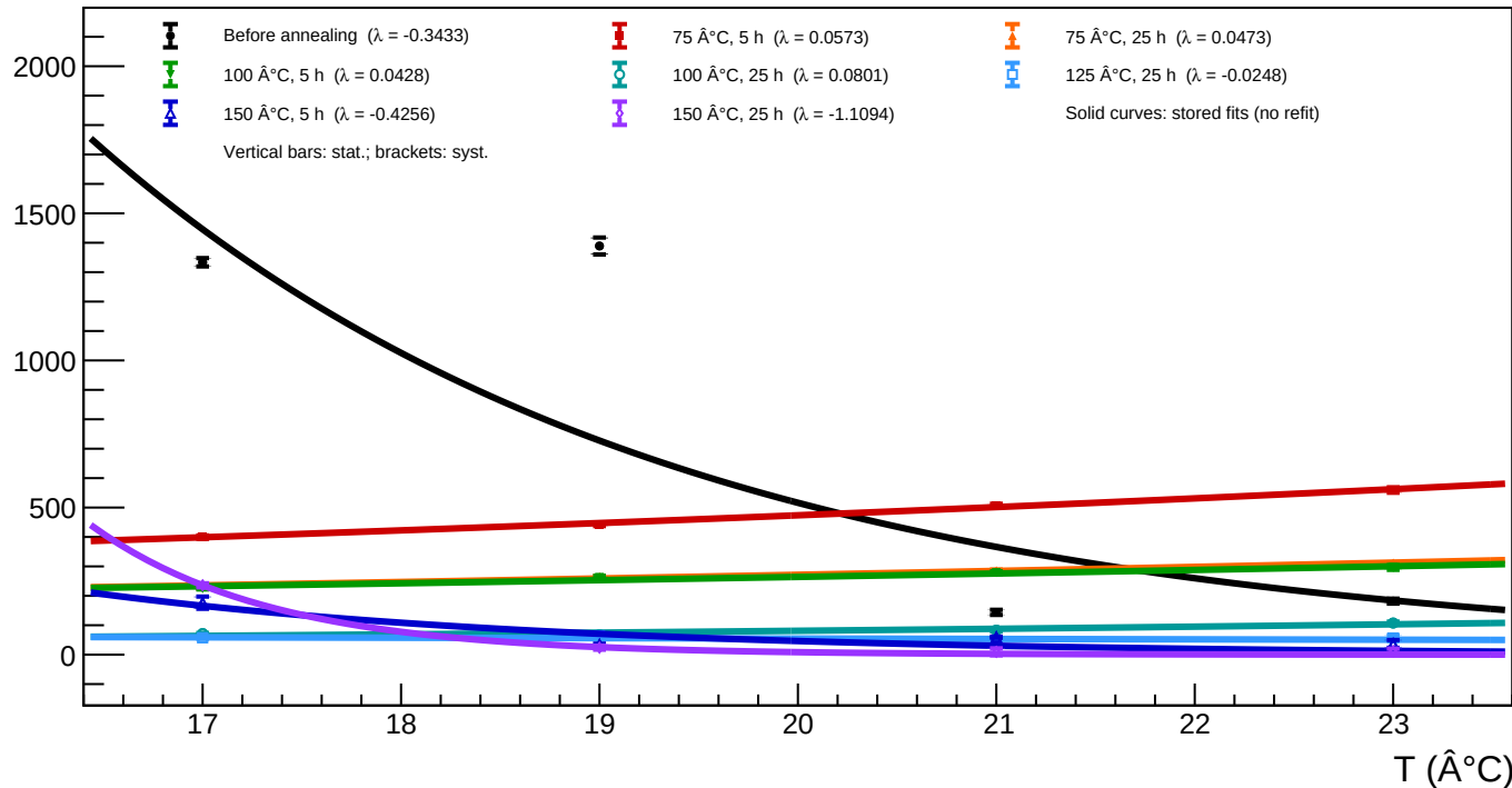
A1_v=5 - Spot 24 ( x = 868.21 , y = 1006.40 ): luminosity vs temperature for all annealing phases
