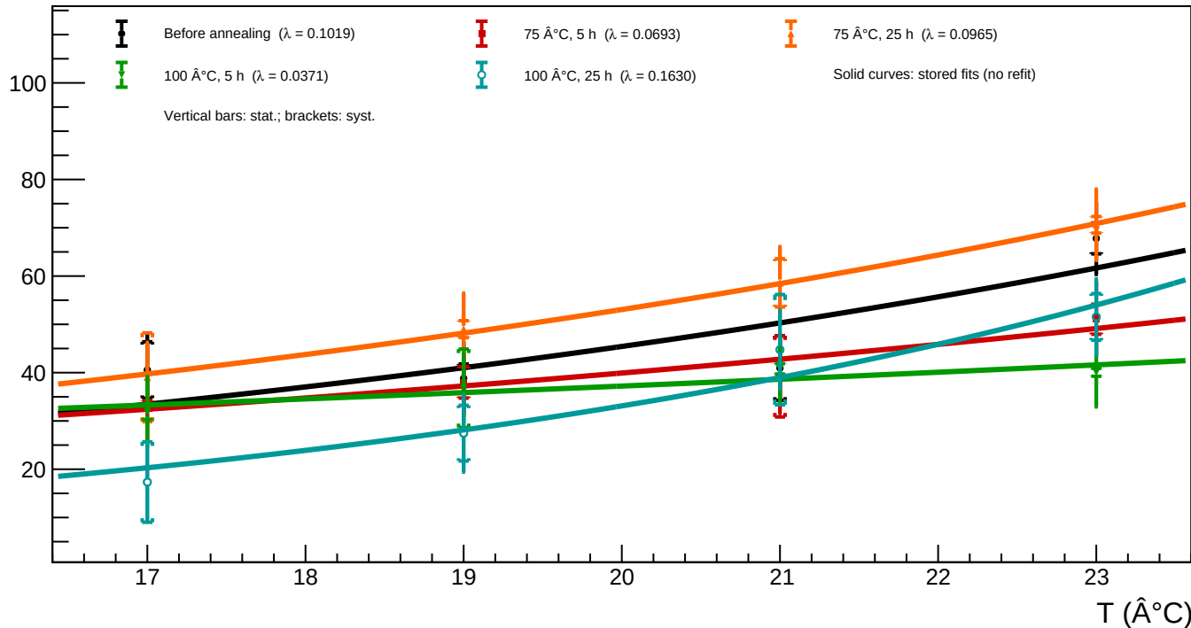
A1_v=5 - Spot 26 ( x = 1006.99 , y = 121.98 ): luminosity vs temperature for all annealing phases
