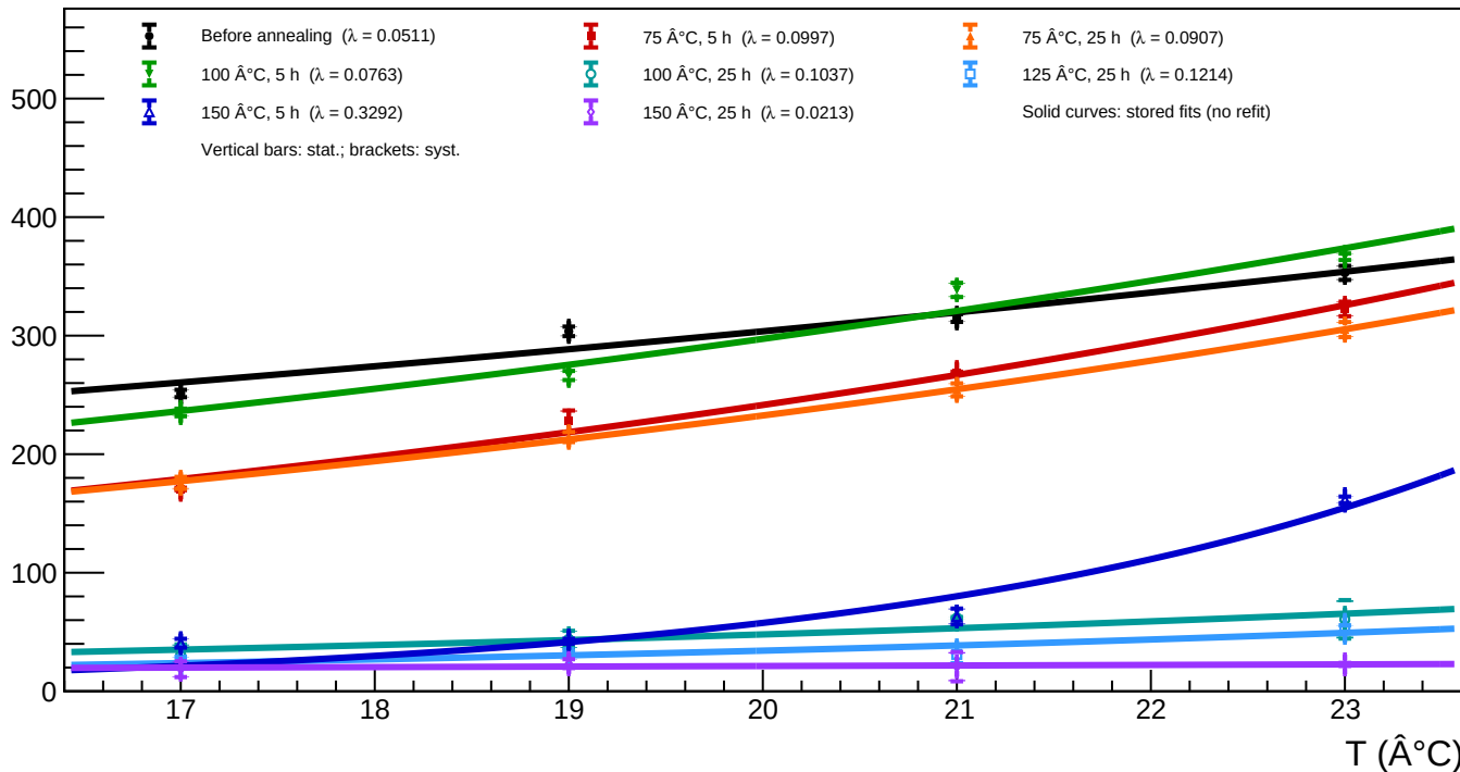
A1_v=5 - Spot 27 (x = 1048.21, y = 956.05): luminosity vs temperature for all annealing phases
