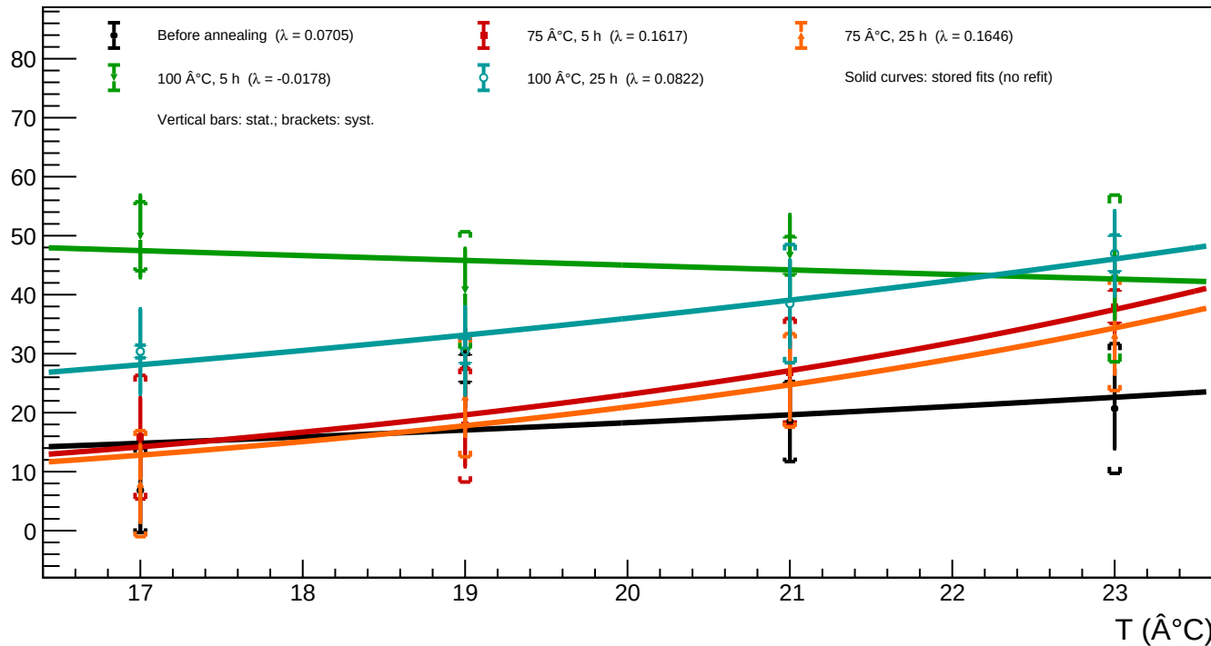
A1_v=5 - Spot 29 ( x = 1068.35 , y = 233.38 ): luminosity vs temperature for all annealing phases
