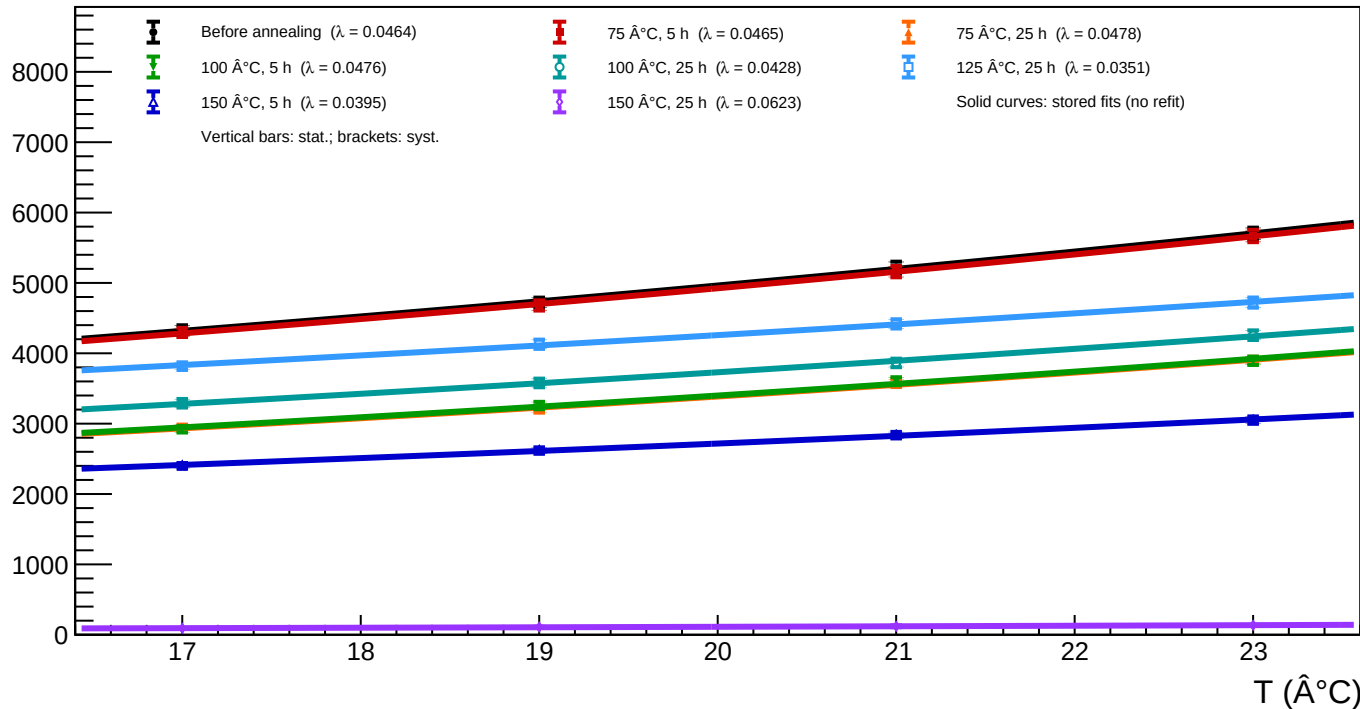
A1_v=5 - Spot 3 ( x = 182.89 , y = 170.30 ): luminosity vs temperature for all annealing phases
