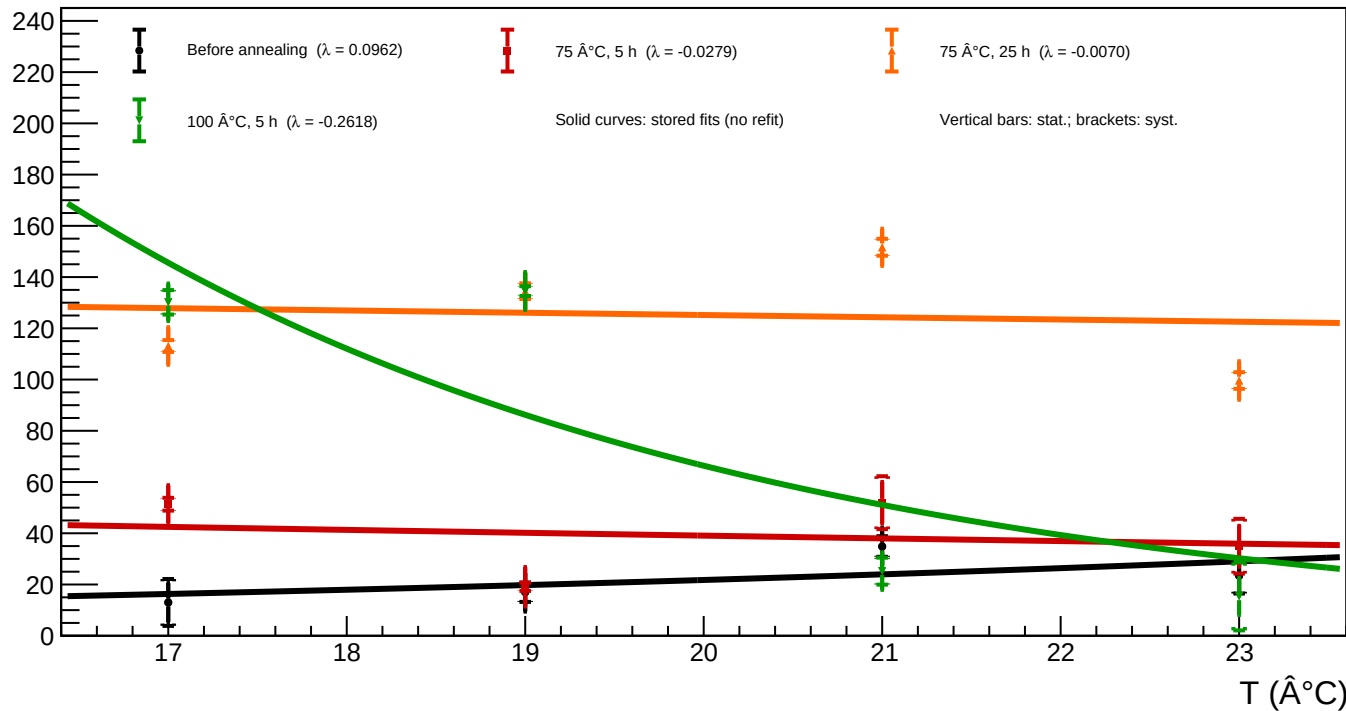
A1_v=5 - Spot 30 ( x = 1087.38 , y = 909.52 ): luminosity vs temperature for all annealing phases
