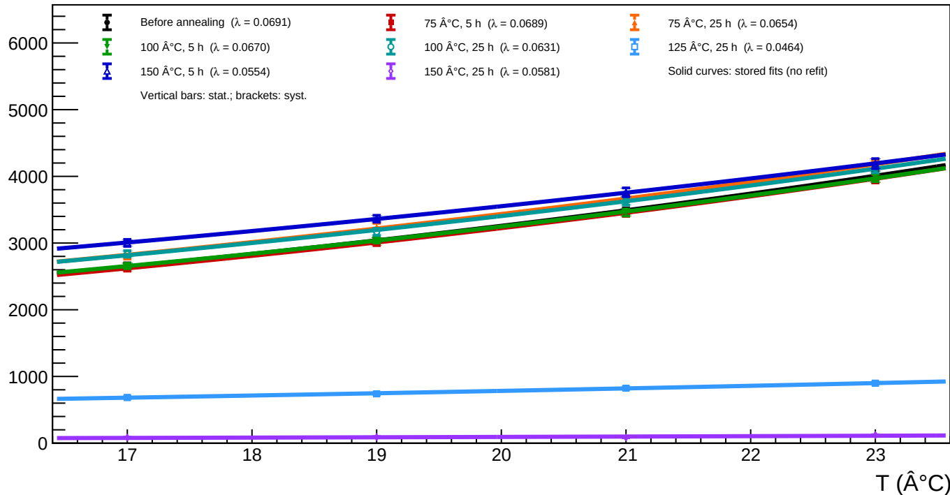
A1_v=5 - Spot 33 (x = 1169.84, y = 238.86): luminosity vs temperature for all annealing phases
