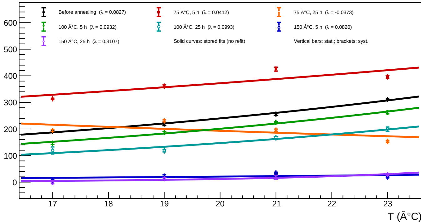
A1_v=5 - Spot 37 ( x = 1244.71 , y = 483.32 ): luminosity vs temperature for all annealing phases
