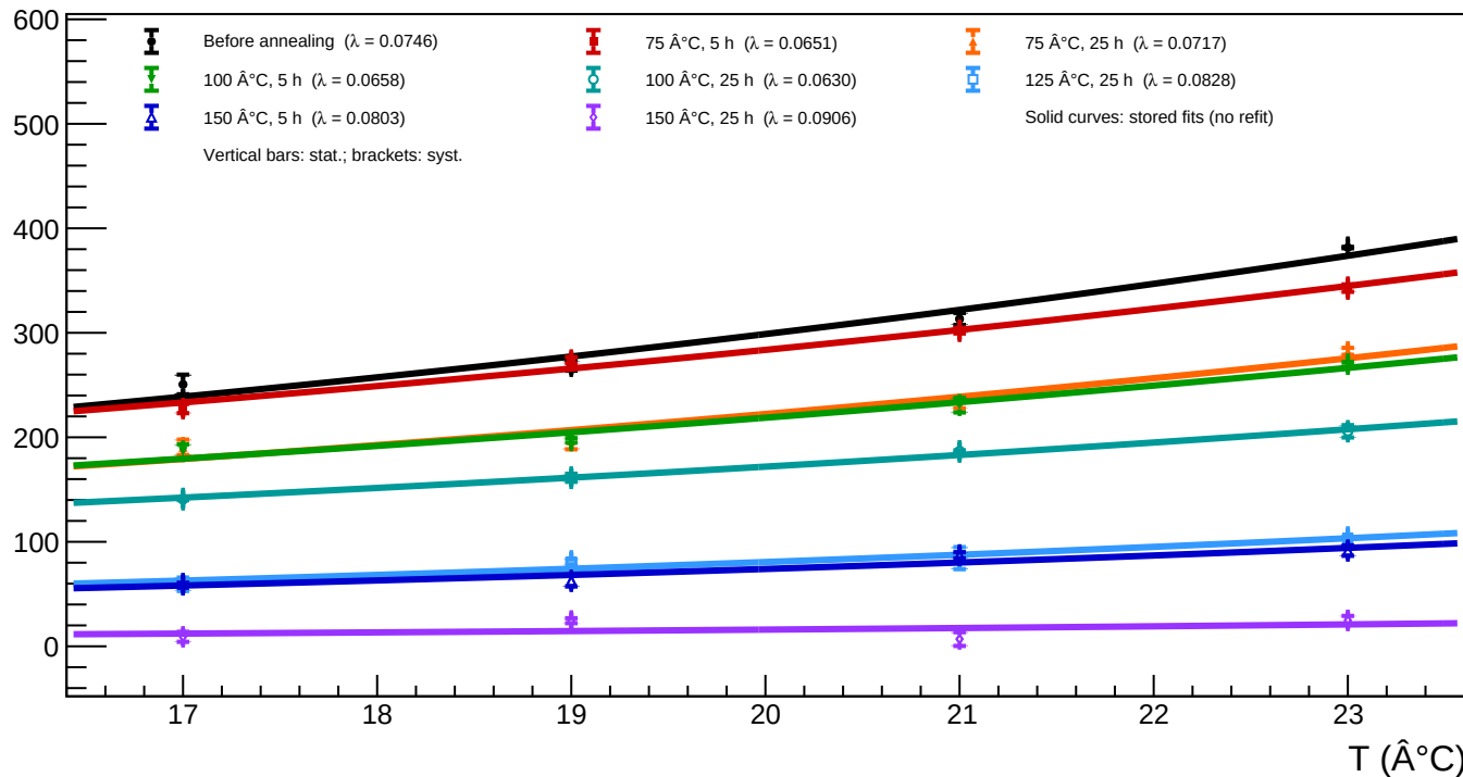
A1_v=5 - Spot 4 ( x = 193.76 , y = 518.45 ): luminosity vs temperature for all annealing phases
