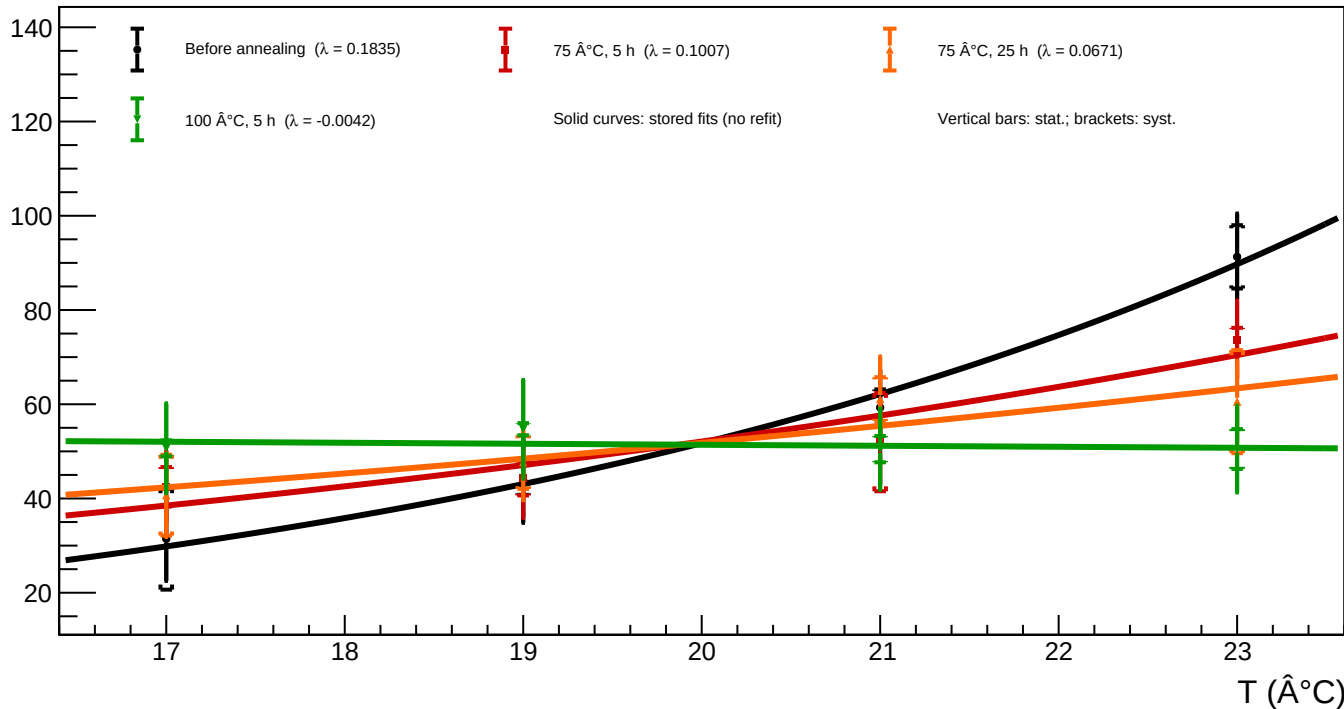
A1_v=5 - Spot 41 ( x = 1287.27 , y = 873.45 ): luminosity vs temperature for all annealing phases
