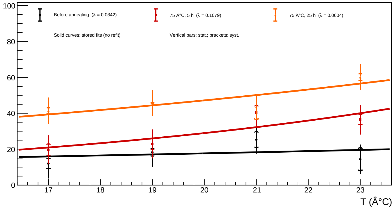
A1_v=5 - Spot 44 (x = 1322.55, y = 529.20): luminosity vs temperature for all annealing phases
