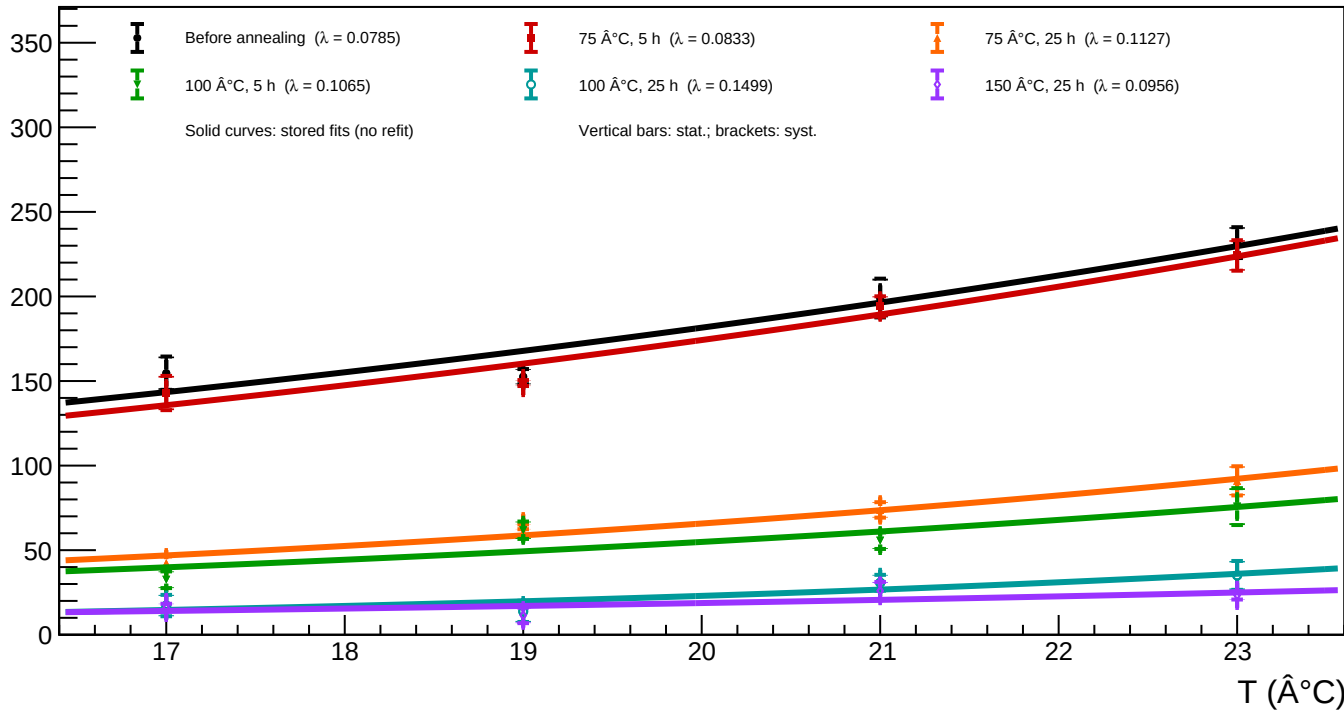
A1_v=5 - Spot 49 (x = 1502.26, y = 863.42): luminosity vs temperature for all annealing phases
